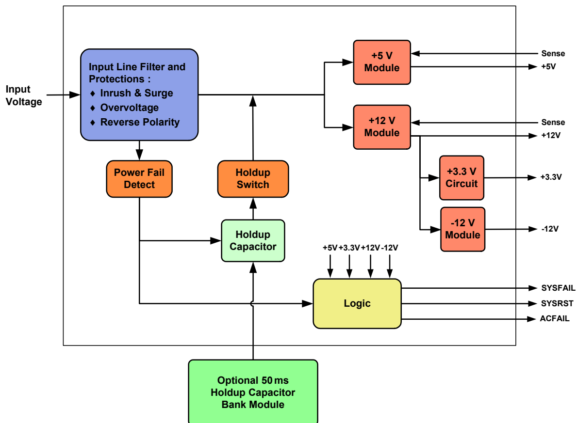
P231 Power Supply Block Diagram
